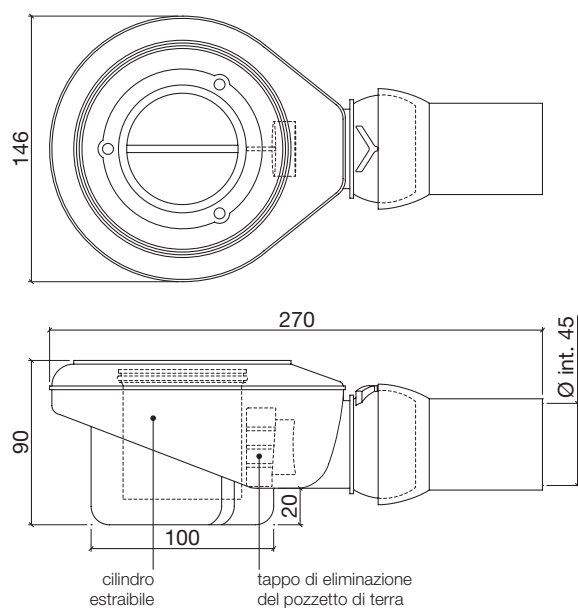
SIFONE PLUS *misure in mm.
