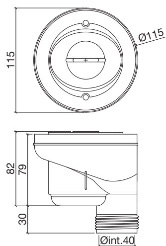
SIFONE VERTICALE *misure in mm.
