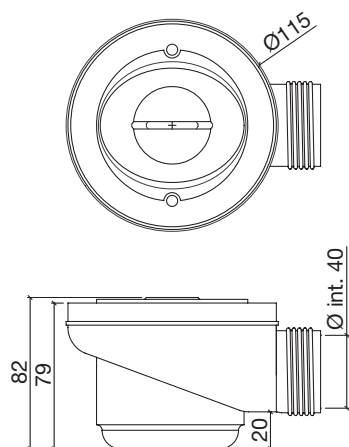
SIFONE ESSENTIAL (STANDARD) *misure in mm.
